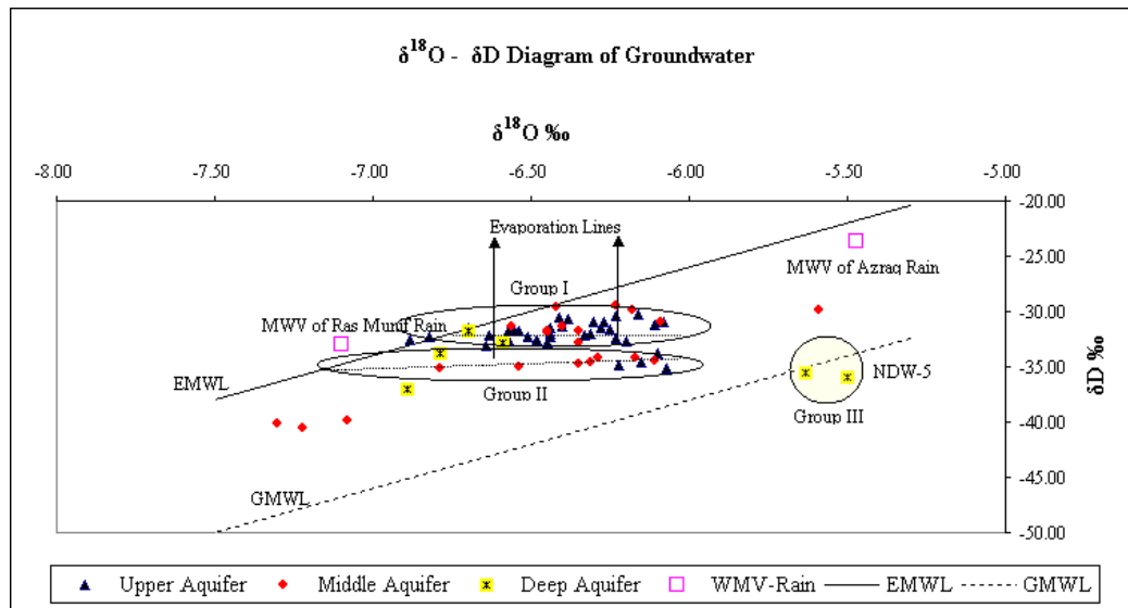
Fig. 9 \delta^{18}\text{O} and \delta\text{D} Diagram of the Azraq Groundwater and Precipitation
