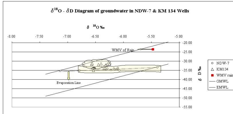
Fig. 9 δ 18 O and δD Diagram of NDW-7 & KM 134 Groundwater Wells
