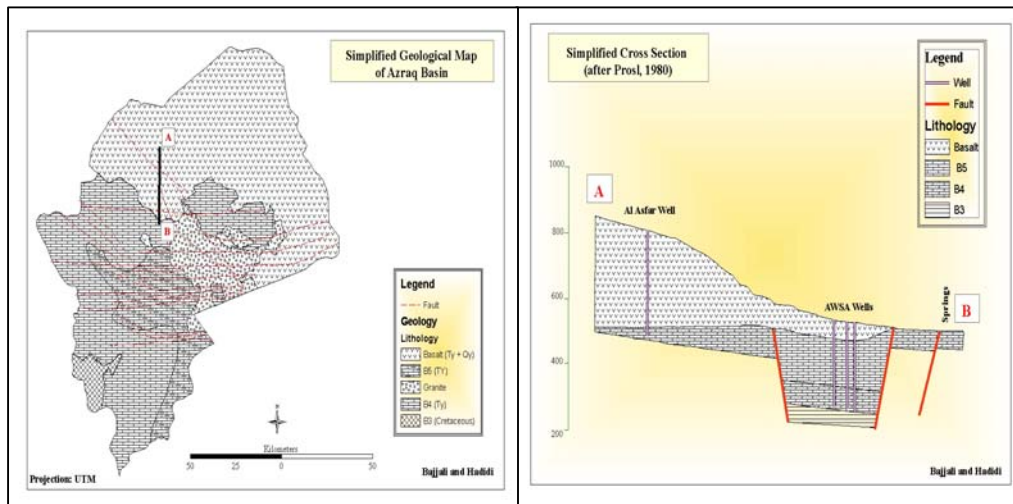
Fig. 2 Simplified Geological Map of Azraq Basin
